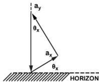
Dual-Axis Tilt Theory Diagram
